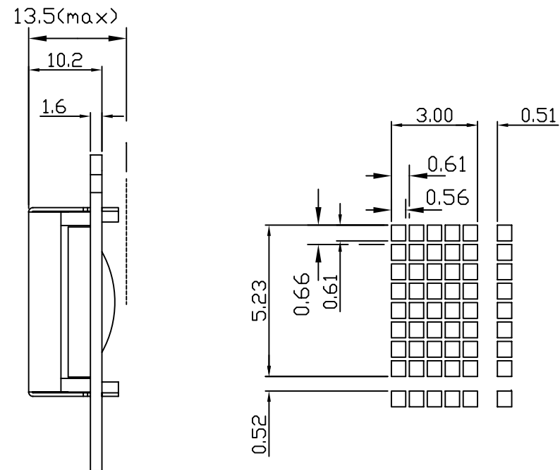
LED BKL Display Pattern
